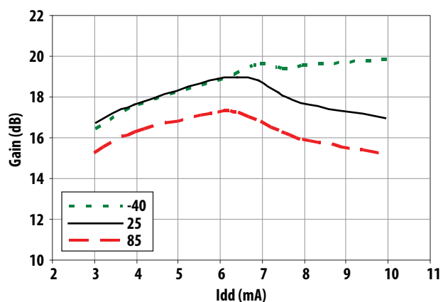
Figure 10. Gain vs. Idd at Vdd = 2.8V
