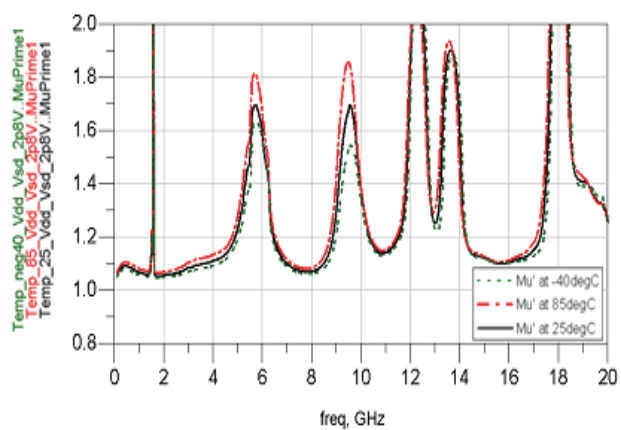
Figure 19. Edwards-Sinsky Input Stability Factor (Mu') at Vdd = 2.8V
