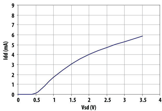
Figure 7. Idd vs Vsd for Vdd = 1.8V, R2 = 3.9k 0hm
