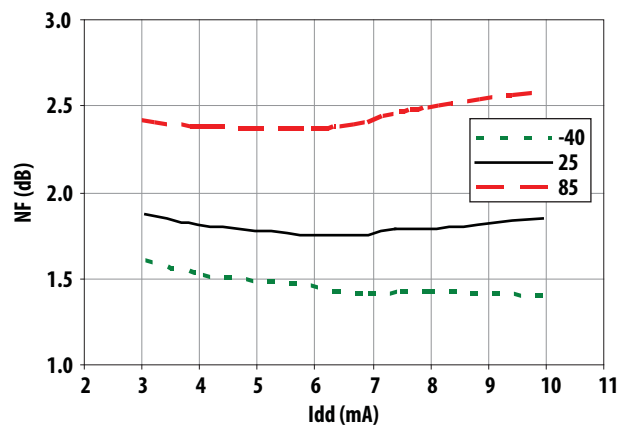
Figure 8. NF vs. Idd at Vdd = 2.8V
