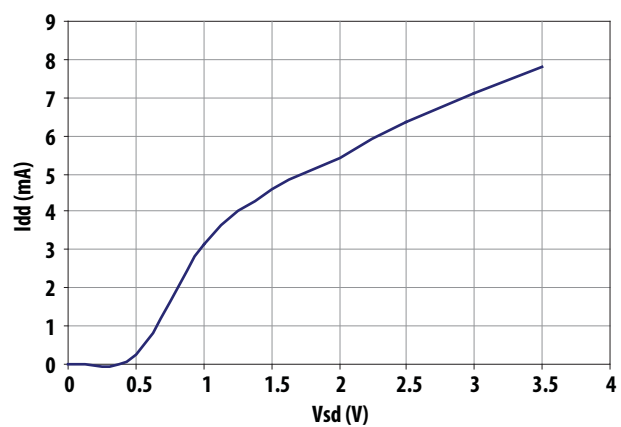
Figure 6. Idd vs Vsd for Vdd = 2.8V, R2 = 3.9k 0hm
