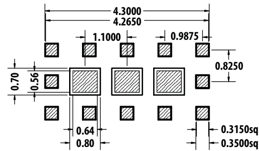
Combined Land Pattern & Stencil Opening
